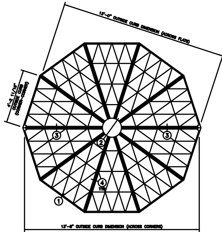
GEO ROOF PLAN NOTE: SHIPPED IN 2 UNITS
