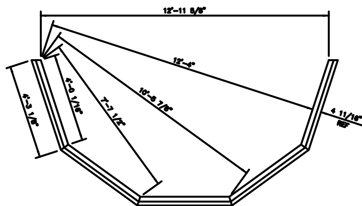
INSTALLATION DIMENSIONS FOR CURB CAP LAYOUT OF HALF THE GEO ROOF
