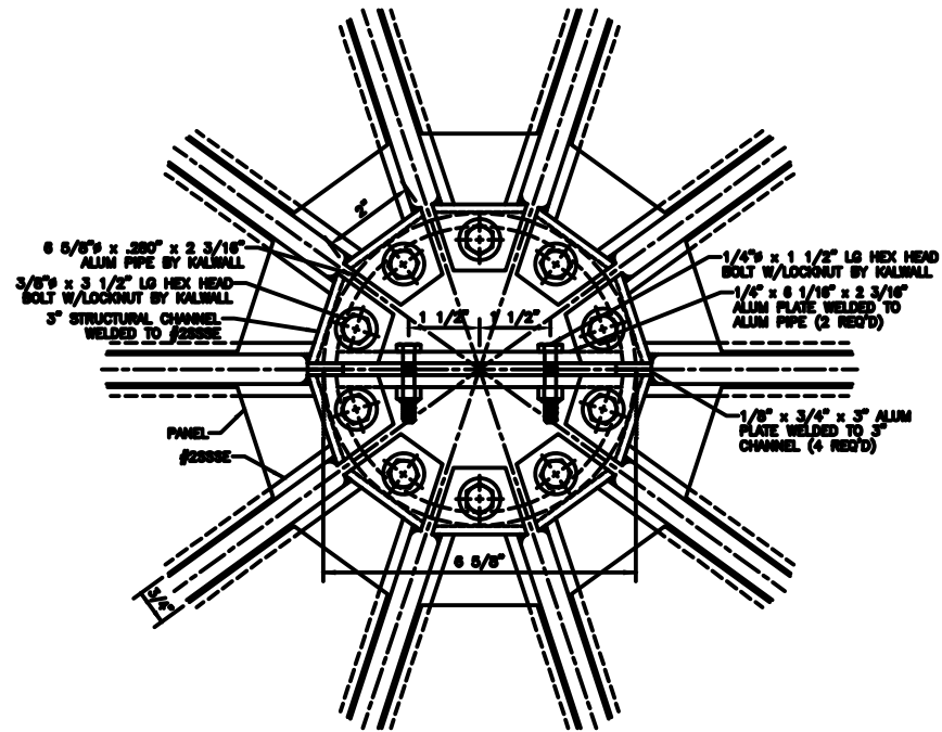
AA COMPRESSION RING PLAN VIEW
