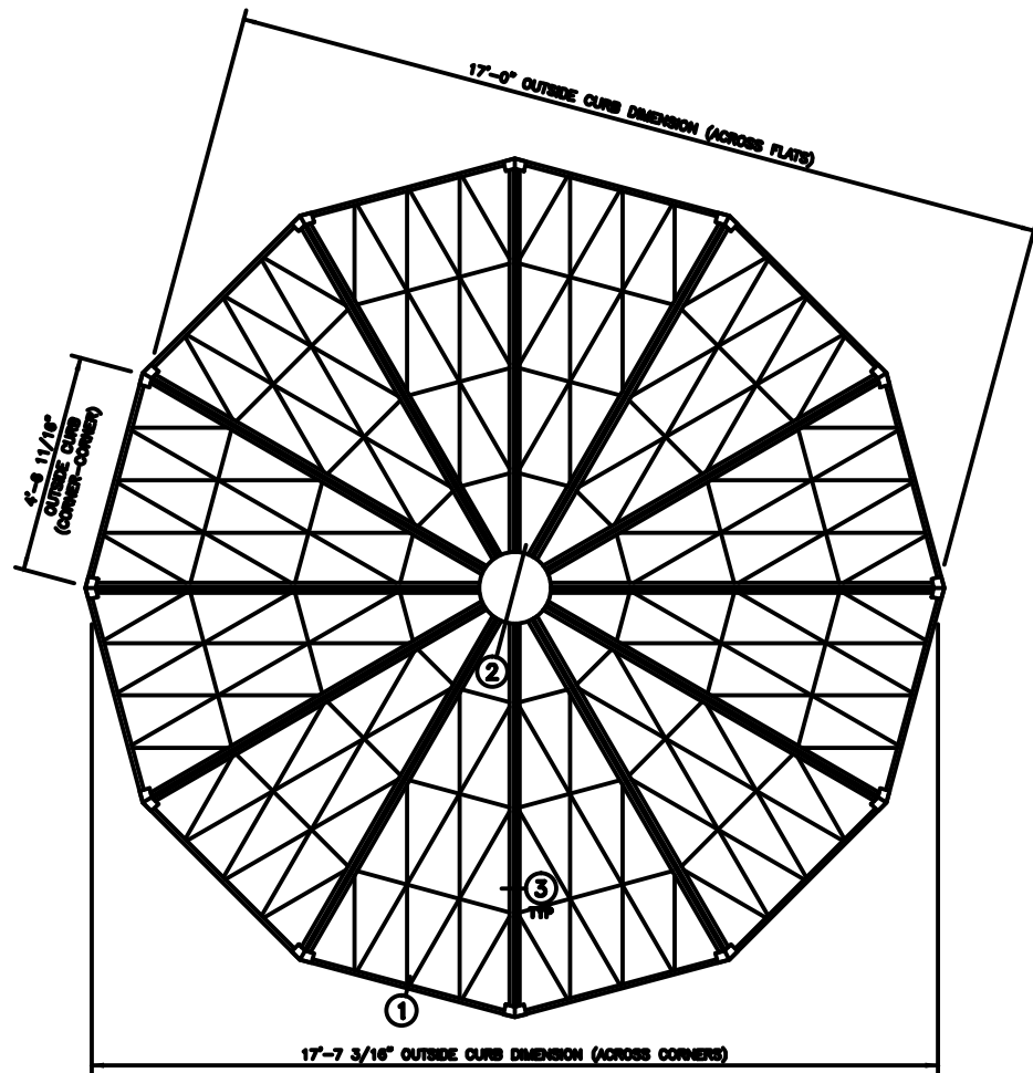
GEO ROOF PLAN NOTE: SHIPPED IN 12 UNITS
