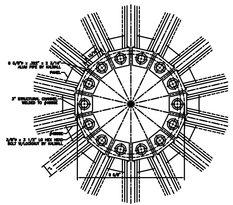
AA COMPRESSION RING PLAN VIEW
