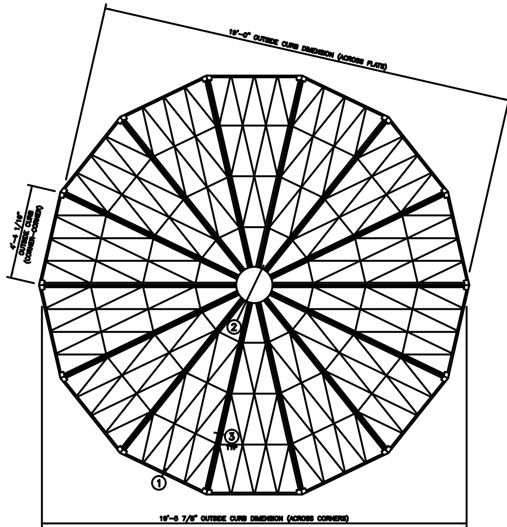
GEO ROOF PLAN NOTE: SHIPPED IN 14 UNITS
