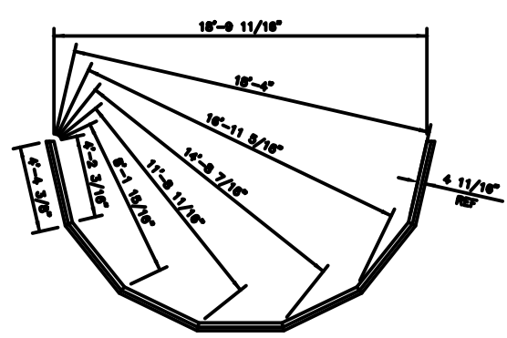
INSTALLATION DIMENSIONS FOR CURB CAP LAYOUT OF HALF THE GEO ROOF
