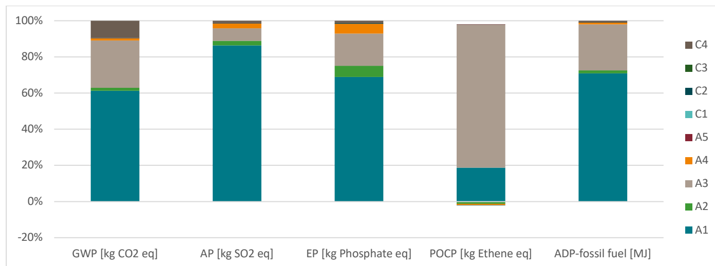
Figure 2: Relative LCIA Results, Wall Panel, TB
