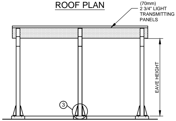
TYPICAL ELEVATION
