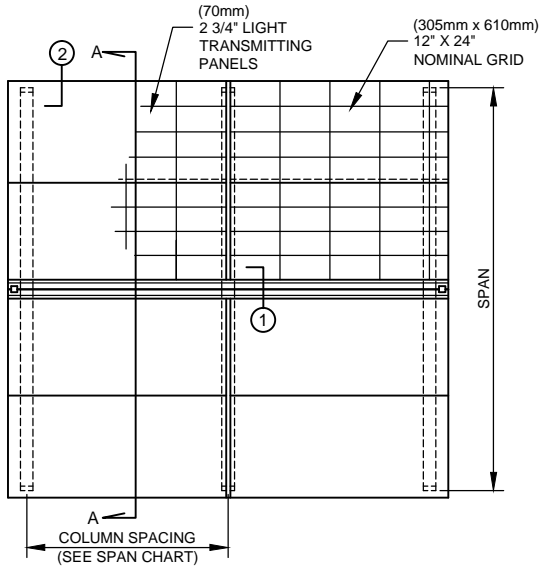
ROOF PLAN
